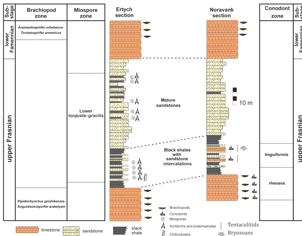
Figure 3. Litho-, bio-, chronostratigraphic correlations of the Ertych and Noravank sections, synthesizing all the currently existing fossil data.
