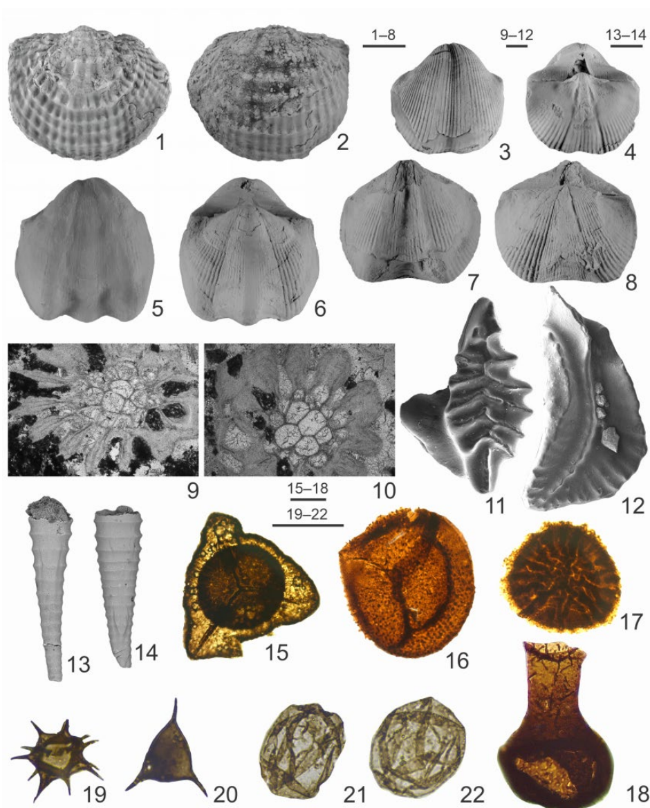
Figure 4. Upper Frasnian and lower Famennian fossils from Central Armenia. 1–2. Spinatrypa sp., almost complete specimen in ventral (1) and dorsal (2) views; IGSNASRAGM 3937/PS 3043, Ertych section, upper Frasnian. 3–4. Angustisulcispirifer arakelyani Serobyan et al., partly exfoliated specimen in ventral (3) and dorsal (4) views; IGSNASRAGM 3972/AR 3078, Ertych section, upper Frasnian. 5–6. Aramazdospirifer orbelianus (Abich), neotype, almost complete specimen in ventral (5) and dorsal (6) views; IGSNASRAGM 3897/AB97/48, Noravank section. 7–8. Tornatospirifer armenicus (Abrahamyan), neotype, partly exfoliated specimen in ventral (7) and dorsal (8) views; IGSNASRAGM 3981/PS 3087, Shamamidzor section. 9. Bigeyella indigena (Morozova and Weiss in Morozova et al.), oblique thin section; Nv17/9h, upper Frasnian. 10. Euthyrhombopora tenuis Ernst et al., branch transverse section; Nv17/9v, upper Frasnian. 11. Icriodus iowaensis iowaensis Youngquist and Peterson; IGS-C23, sample Nv23/2, upper Frasnian. 12. Polygnathus webbi Stauffer; IGS-C5, sample Nv23/2, upper Frasnian. 13–14. Tentaculitidae gen. et sp. indet., specimen in ventral (13) and dorsal (14) views; sample Nv19/134, Noravank section, lower Famennian. 15. Teichertospira torquata (Higgs) McGregor and Playford; sample Er18/P13, Q68/2, lower Famennian. 16. Acinosporites lindlarensis Riegel; sample Er18/P7, G14/4, lower Famennian. 17. Kraeuselisporites ollii McGregor and Camfield; sample Er18/P2, X11/2, lower Famennian. 18. Angochitina mourai Lange; sample Er18/P2, D50, lower Famennian. 19. Michrhystridium stellatum Deflandre; sample Er17/12/3, T51, lower Famennian. 20. Gorgonisphaeridium cf. ohioense ; sample Er17/7/1, K71/3, lower Famennian. 21–22. Leiosphaeridia sp.; sample Er17/5/3 (21), B58/4 and sample Er17/5/2 (22), Y61/1, lower Famennian. Scale bars = 10 mm (1–8), 100 µm (9–12), 200 µm (13–14), 20 µm (15–22).
